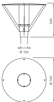
TRANSPARENT ACRYLIC DIFFUSER FOR ø102mm POLE
