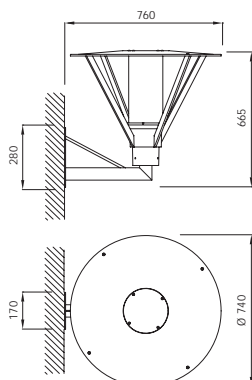
opal (inside) acrylic diffuser
