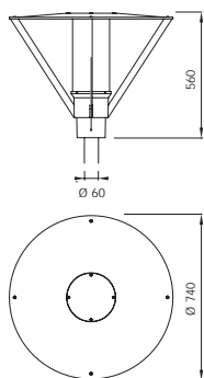
TRANSPARENT ACRYLIC DIFFUSER FOR ø60mm POLE AND WALL BRACKET
